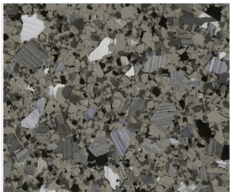
Slate
