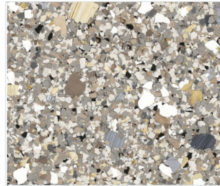
Travertine
