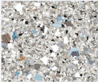
Blue Granite
