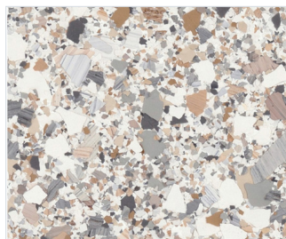
Claystone
