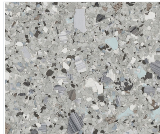
Agate
