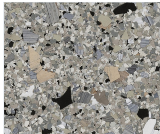
Shale
