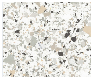
Limestone
